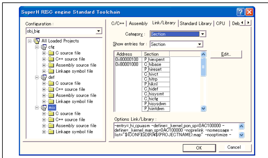
Figure 5.13 Optimized Linkage Editor [Section]
